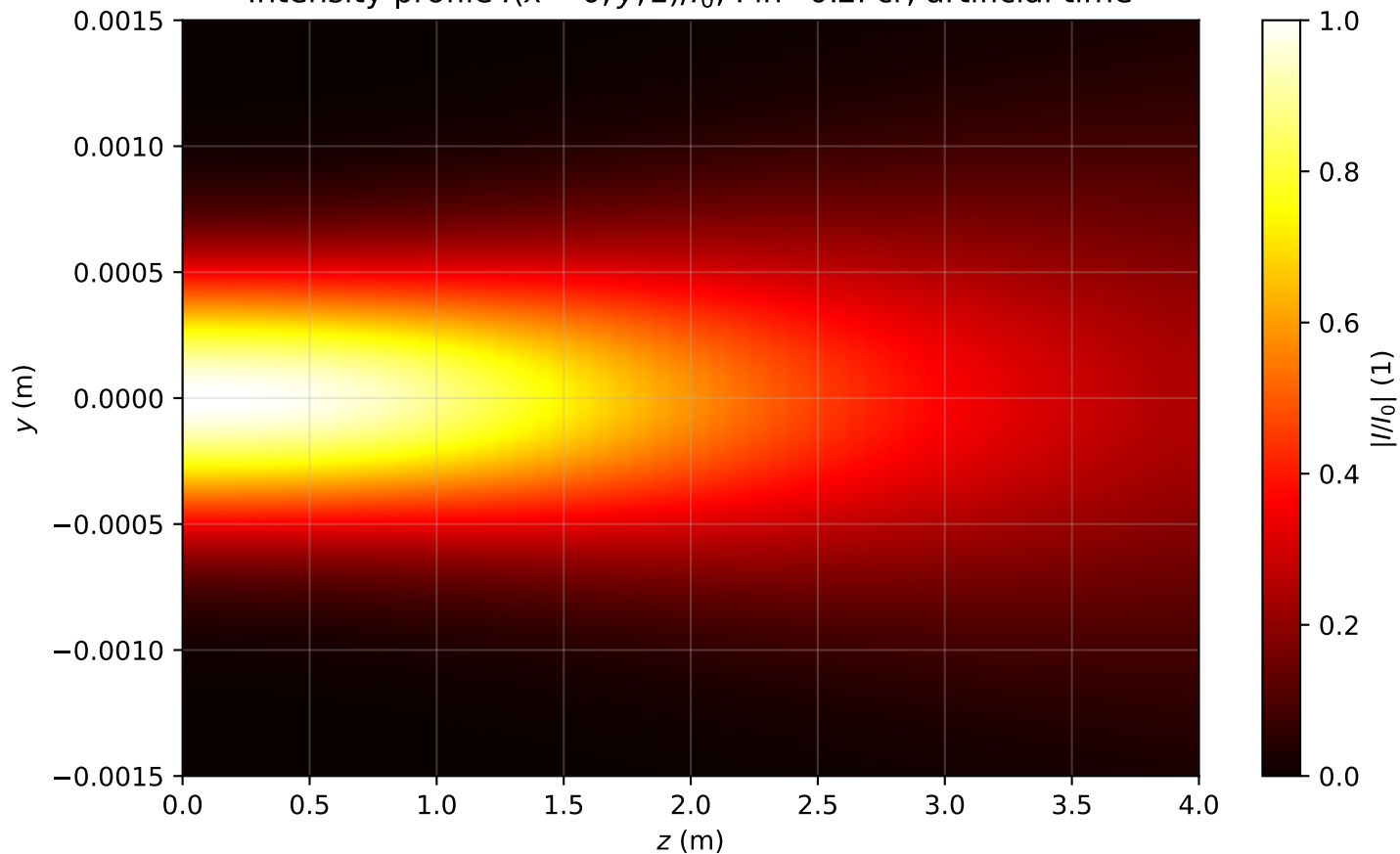
Intensity profile I(x=0, y, z)/I_0 , P_{in}=0.2P_{cr} , artificial time
